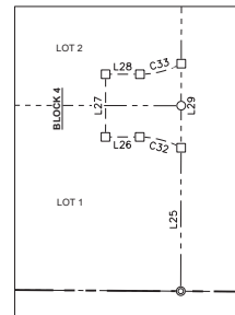
DETAIL "B" - HAMMERHEAD EASEMENT SCALE: 1" = 30'
