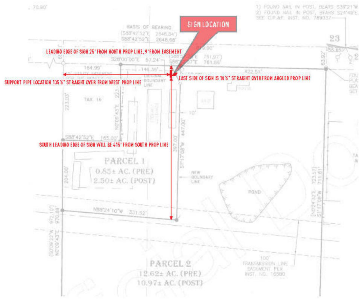
SITE PLAN
